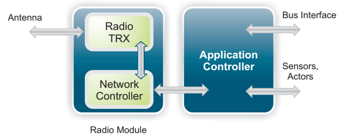
Figure : "Split" Architecture with Network Controller and Application Controller
